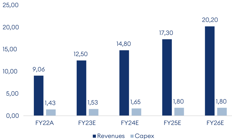
CHART 3 – CAPEX FY22A-26E
